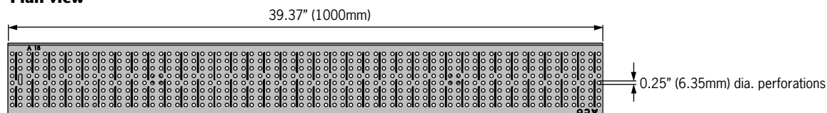
Plan view
